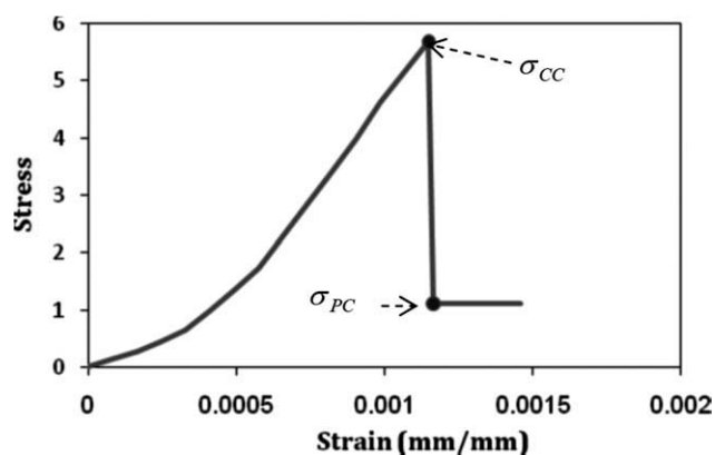
Figure 12 A typical flexural behavior of fiber reinforced cement composite.
