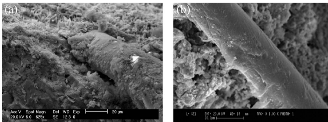
Figure 6 Acrylic fiber embedded in cement matrix; fiber surface covered by cement matrix: (a) wet-spun acrylic fiber and (b) dry-spun acrylic fiber.
